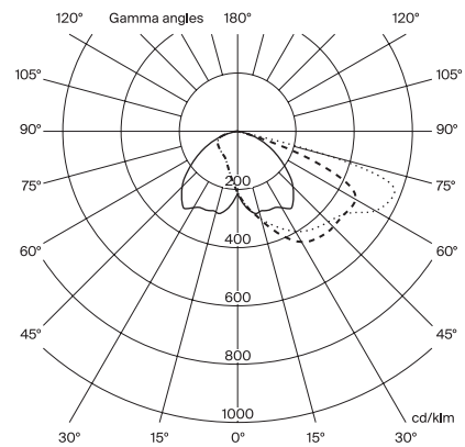
Type routier Distribution TIV LOR 100% ULOR 0%±3%
