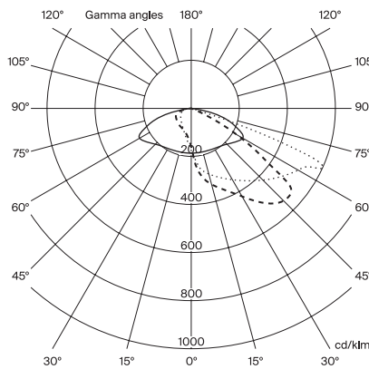
Type routier Distribution TIII LOR 100% ULOR 0%±3%
