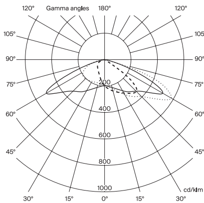
Type routier Distribution TII LOR 100% ULOR 0%±3%
