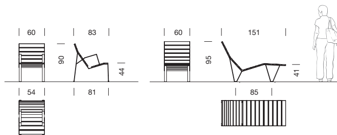
Longue chair 0.60 m
