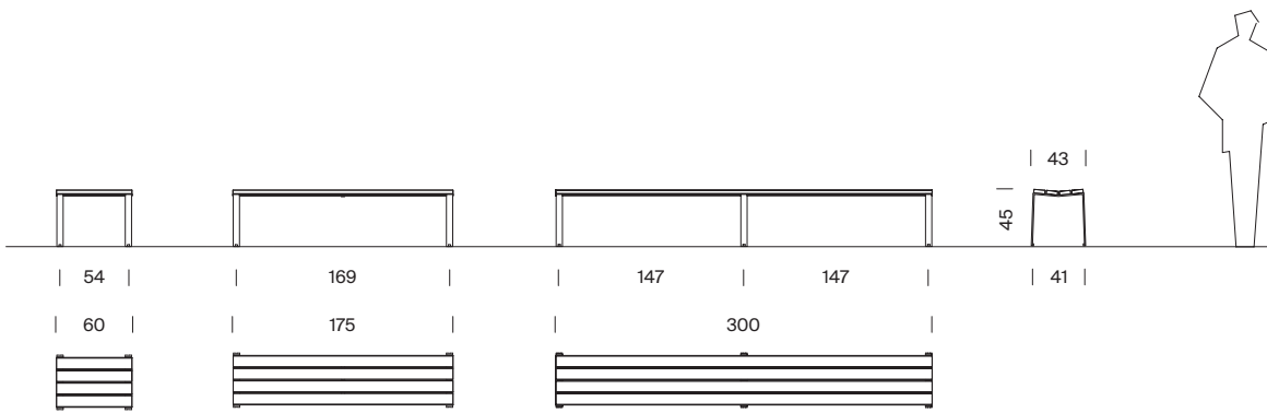
Banquette Harpo 0.60m, 1.75 m and 3.00 m without arms
