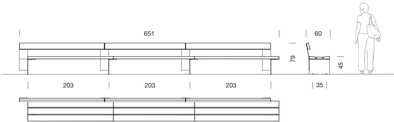
Bancal bench 3 units with 3 backrests
