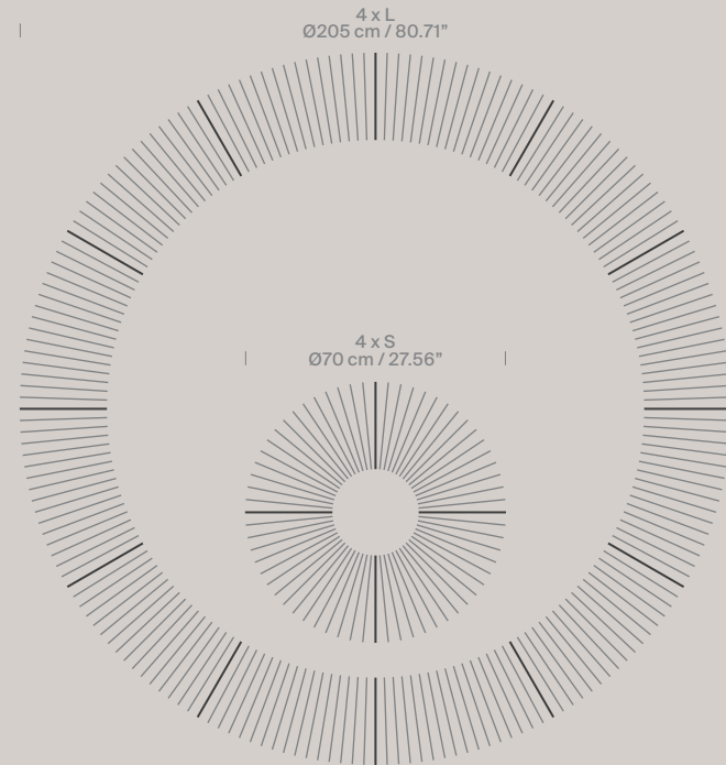
Pendant lamp Upper view
